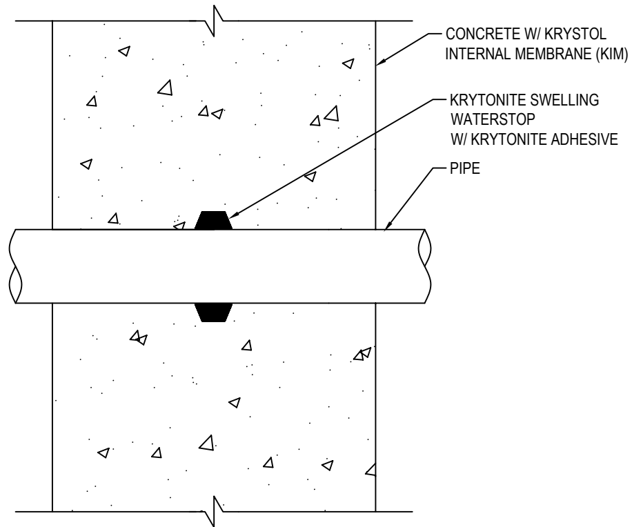
PIPE PENETRATIONS INTERNAL SWELLING METHOD
