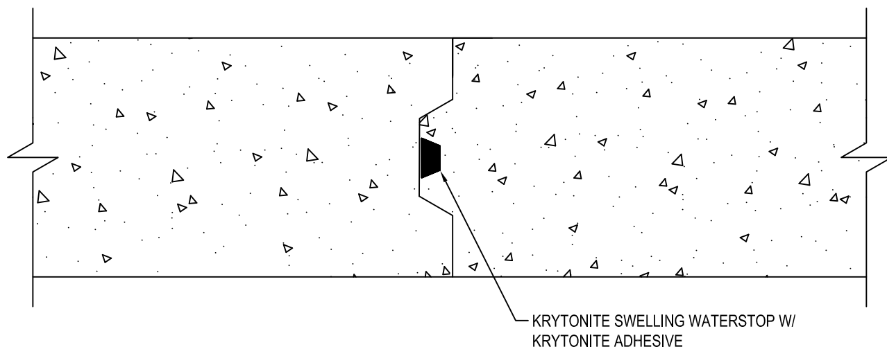
SLAB TO SLAB CONSTRUCTION JOINTS SINGLE PROTECTION
